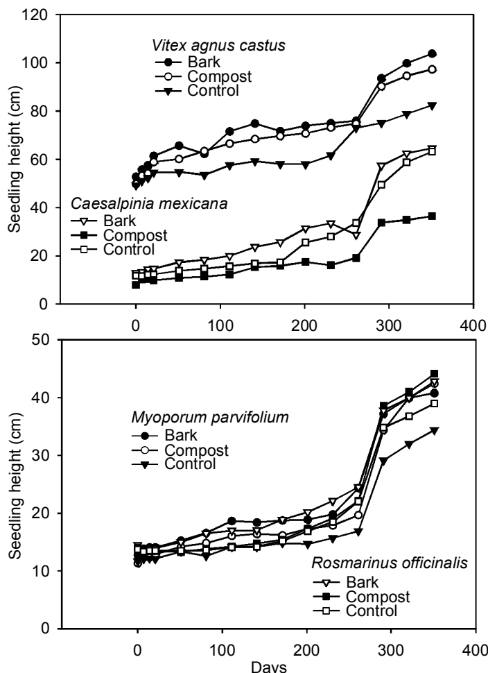
Fig. 2. Seedling height of different species under different mulch treatments. (A) Vitex agnus castus and Caesalpinia mexicana (B) Myoporium parvifolium and Rosmarinus officinalis
